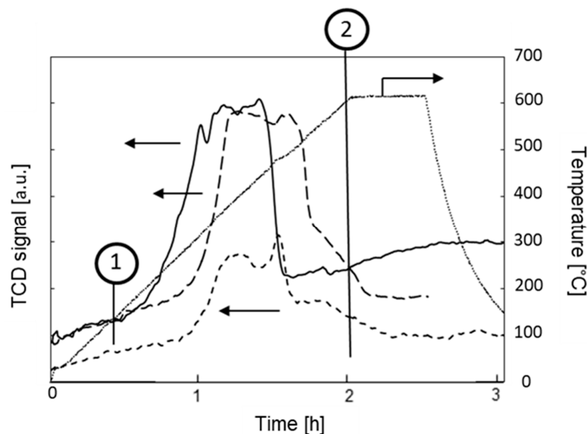
Figure 8. Temperature Programmed Oxidation (TPO) results of the undoped cobalt catalyst (long dashes: 475 mg; short dashes: 210 mg) and \text{Co}_{3.5}\text{La} (solid line: 475 mg) and the function of temperature in time (dotted line); line 1 indicates the onset of oxidation of \text{Co}_{3.5}\text{La} , line 2 indicates the beginning of the isothermal segment.
