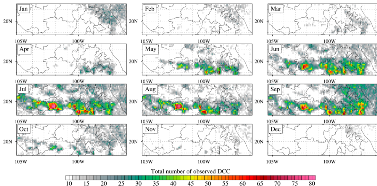
Figure 3. Monthly distribution of the total number of observed deep convective clouds based on MODIS cloud data (2008–2017) with a horizontal resolution of 0.1 degrees.
