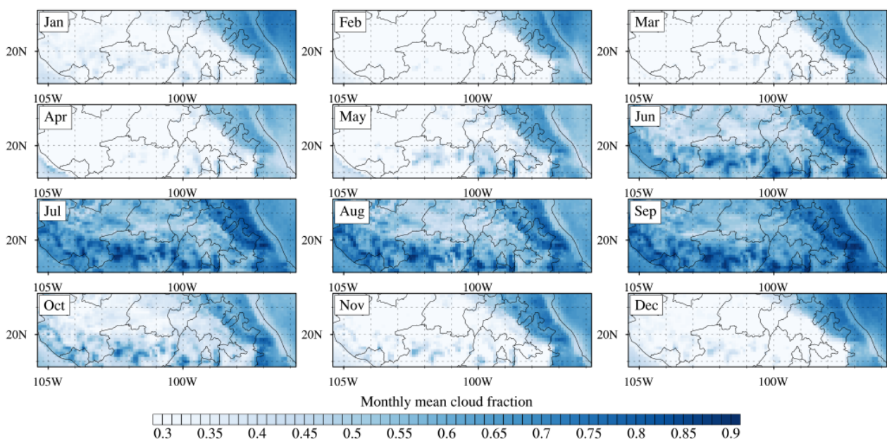
Figure 2. Monthly distribution of mean cloud fraction based on Moderate-Resolution Imaging Spectroradiometer (MODIS) cloud data (2008–2017) with a horizontal resolution of 0.1 degrees.
