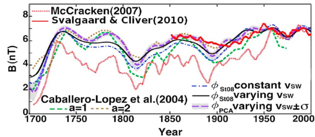
Figure 1. Reconstructions of long-term variations in near-Earth magnetic field intensity, B , over the period 1700–2000, adapted from Svalgaard and Cliver [2010] and Steinhilber et al. [2010]. The solid red line shows a 25 year running mean of the geomagnetic B reconstruction from Svalgaard and Cliver [2010]. Other curves show cosmogenic radionuclide reconstructions of B . They are: 40 year running means ( \Phi_{St08} , blue and black lines) and 25 year running means ( \Phi_{PCA} , purple line) from different heliospheric modulation potential estimates provided by Steinhilber et al. [2010]; 22 year running means of Caballero-Lopez et al. [2004] estimates (green and gold lines); 11 year running means of the McCracken [2007] estimate.
