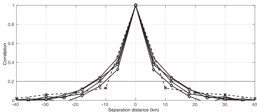
FIG. 7. All elevation along-beam observation error correlation for cases 1 (control; squares), 2 (alternate background error statistics; diamonds), 3 (thinned raw data; triangles), and 4 (new observation operator; circles) and those found previously by Météo-France (crosses). Error correlations are deemed to be insignificant below the horizontal line at 0.2.
