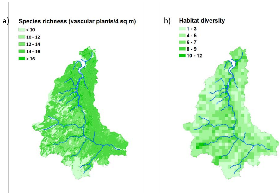
Figure 11. Biodiversity metrics for the Conwy catchment: a) Estimated vascular plant species richness; and b) habitat diversity.
