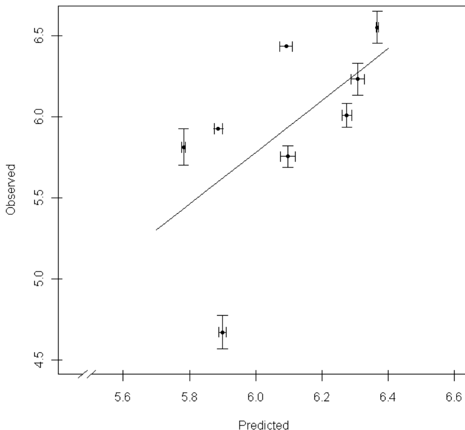
Figure B2. An independent test of observed versus predicted \ln\text{NPP} ( \text{gm m}^{-2} \text{yr}^{-1} ) using subsets of vegetation plots from the GB Countryside Survey in 1998. Observed \ln\text{NPP} in the model training data was compared with \ln\text{NPP} predicted from the empirical model and applied to all plots from the survey that were referable to the same ecosystem types as those represented by the experimental study systems. Each point represents the mean \pm 1 se.
