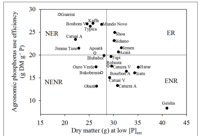
FIGURE 2 | Relationship between shoot dry matter (DM) at low P and responsiveness to P, measured as agronomic phosphorus (P) use efficiency for different coffee cultivars. Coffea arabica (closed symbols) and C. canephora (open symbols). Solid lines represent the mean value for the axis. NER, non-efficient and responsive; ER, efficient and responsive; ENR, efficient and non-responsive; NENR, non-efficient and non-responsive.
