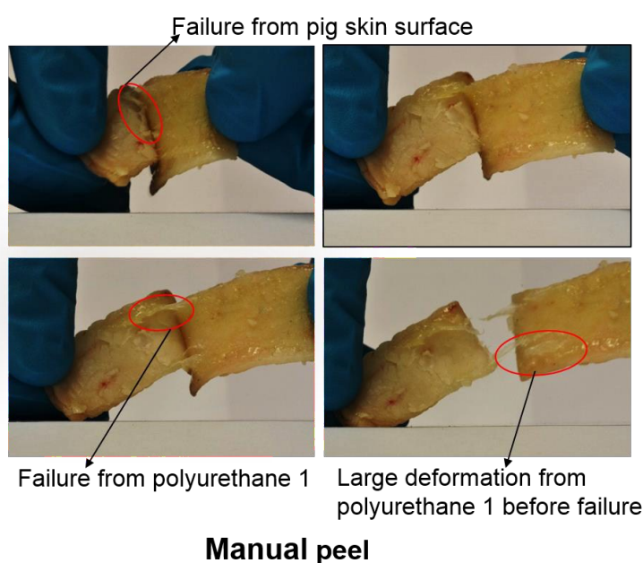
Fig. 7 The investigation of the adhesive property of polyurethane 1 with a pig skin substrate.
