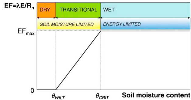
Figure 6. Definition of soil moisture regimes and corresponding evapotranspiration regimes. EF denotes the evaporative fraction (ratio of latent heat to net radiation), EF_{max} its maximum value. Reprinted from Seneviratne et al. [2010] with permission from Elsevier.
