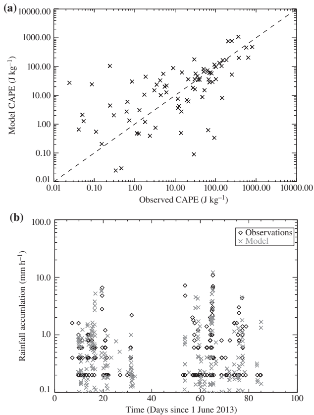
Figure 3. Model and observations comparisons showing (a) a scatter plot for the CAPE at Camborne for JJA 2013, showing all data except where either model or observed CAPE are zero, with a 1:1 line, and (b) a time series comparison of hourly precipitation accumulations at Camborne for JJA 2013, with observations in black and model in grey.
