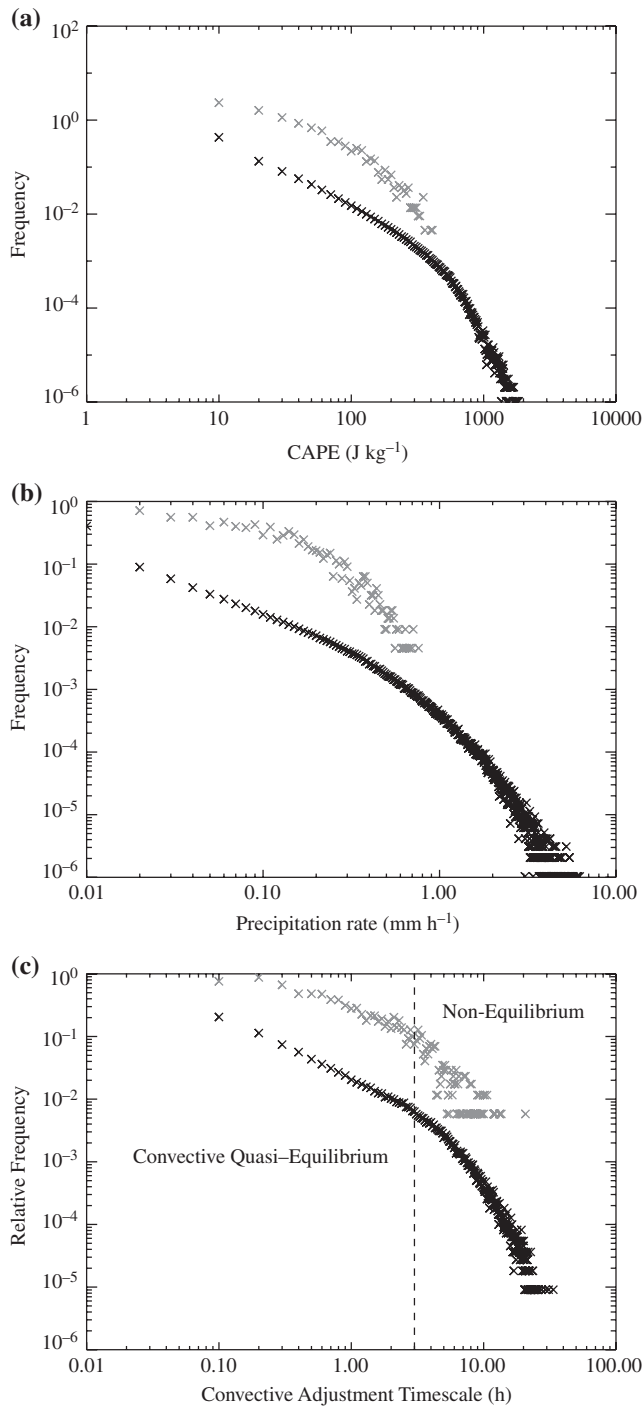
Figure 4. Frequency distributions for the UKV domain showing (a) CAPE, (b) precipitation rate (no thresholding applied) and (c) the convective adjustment timescale (calculated using thresholded precipitation) for JJA 2012–2014 as an average over the coarse-grained UKV model output (grey) and over all coarse-grained points in the domain (black). Bin sizes are 10 \text{ J kg}^{-1} for CAPE, 0.01 \text{ mm h}^{-1} for precipitation and 0.1 \text{ h} for convective adjustment timescale. Frequency is shown normalised by the total number of events—the maximum possible number of events is 92 \text{ days} \times 3 \text{ years} \times 8 \text{ time periods per day} (UKV domain average) and 92 \text{ days} \times 3 \text{ years} \times 8 \text{ time periods per day} \times 440 \text{ grid points} (all points in UKV domain), but zero values and undefined values (the timescale is undefined for zero precipitation) are not shown. The distributions for the UKV domain average in each plot have been shifted upwards by an order of magnitude to allow easier comparison.
