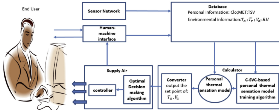
Fig. 8. The Structure and Information flow of PCS System with C-SVC Algorithm.
