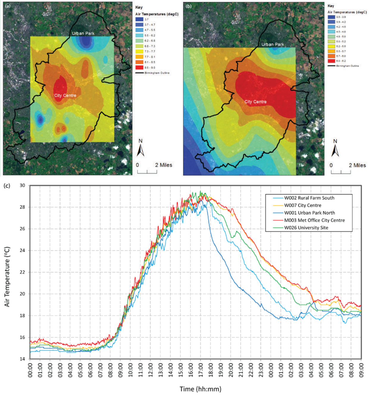
FIG. SBI. (a) Interpolated UHI map at 0100 LT 6 May 2013 (based on available data from 18 sensors) plus aerial imagery, (b) interpolated UHI map at 0100 LT 19 Feb 2014 (based on available data from 23 sensors) plus aerial imagery (source: OpenStreetMap), and (c) diurnal air temperatures during one day of the 22–23 Jul 2013 heatwave.
