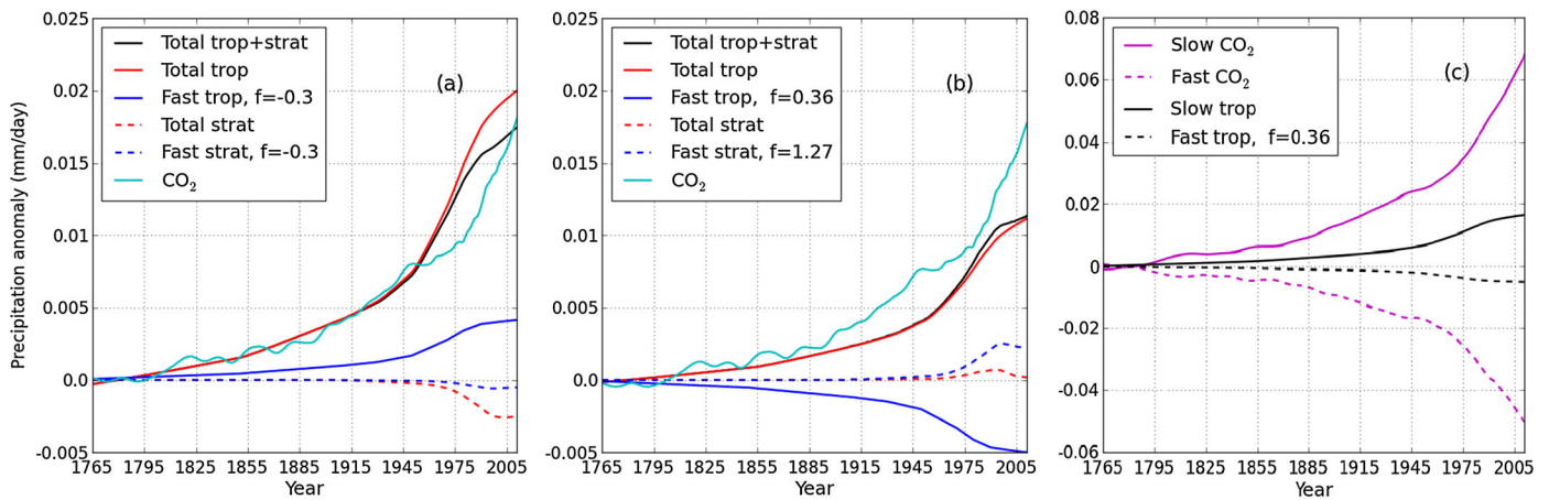
Figure 3. Simple model estimates of the global-mean precipitation response to ozone forcing using the IPCC AR5 radiative forcings from 1765 to 2010. (a) Total and fast precipitation response to tropospheric, stratospheric ozone and both using f = -0.3 . The total response to \text{CO}_2 is also shown. (b) As in Figure 3a but using f = 0.36 for tropospheric and f = 1.27 for stratospheric ozone. (c) The fast and slow components of the response for \text{CO}_2 and tropospheric ozone.
