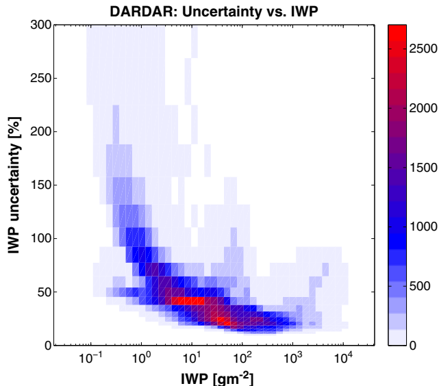
Figure 2. The fractional uncertainty of IWP (%) as a function of IWP for DARDAR.
