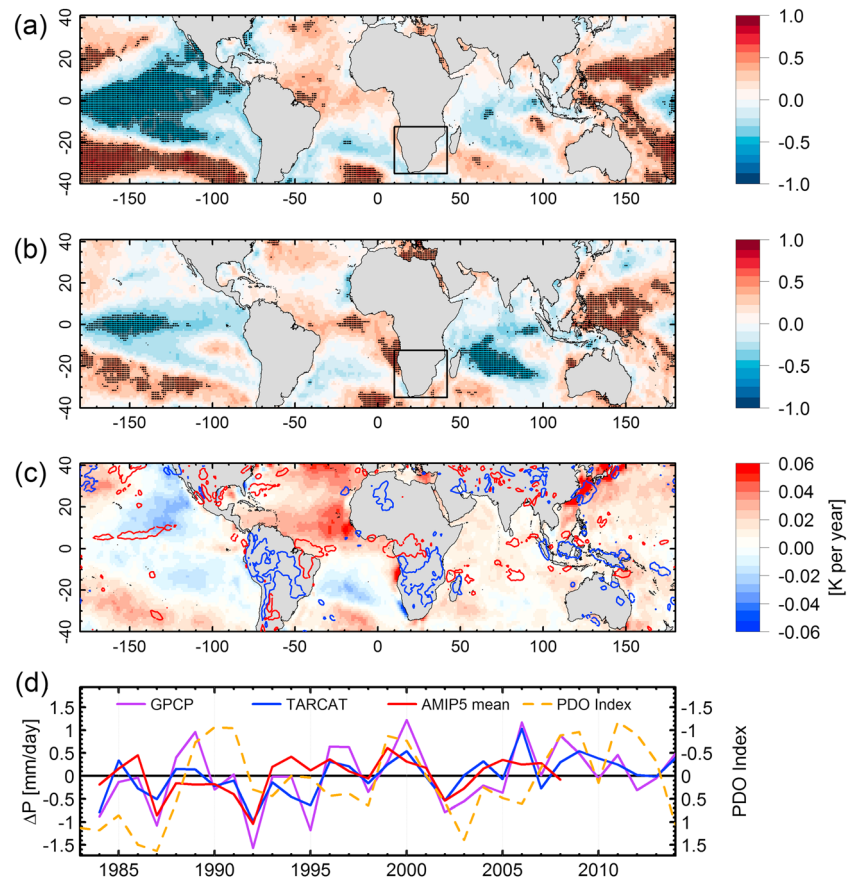
Figure 4. Correlation between DJF mean SST and DJF Southern Africa rainfall (1983–2008) from (a) TARCAT and (b) AMIP5 ensemble mean (stippling indicates statistically significant ( P < 0.05 ) correlations), (c) 1983–2008 trends in DJF SST (shading) and vertical velocity (given by contours of \pm 80 \text{ Pa d}^{-1} \text{ yr}^{-1} ) derived from mean monthly ERA-Interim 500 hPa reanalysis fields (blue contours indicate regions of increased ascent; while red contours indicate regions of decreased ascent), and (d) time series of observed Southern Africa rainfall anomalies and PDO index ( http://research.jisao.washington.edu/pdo/PDO.latest ) for DJF (year corresponding to January).
