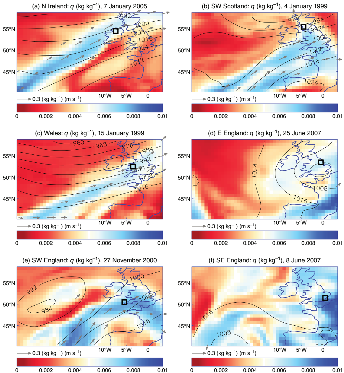
Figure 3. ERA Interim 850 hPa specific humidity ( \text{kg kg}^{-1} , colours) and water vapour transport [arrows, plotted for V_T > 0.1 ( \text{kg kg}^{-1})(\text{m s}^{-1}) ] associated with the heaviest daily rainfall event in the GPCP-1DD record over the period 1997–2008 (date plotted) over regions denoted by \square : (a) Northern Ireland, (b) Southern Scotland, (c) Wales, (d) Eastern England, (e) South West England and (f) South East England. Contours of daily pressure fields at mean sea level are over-plotted.
