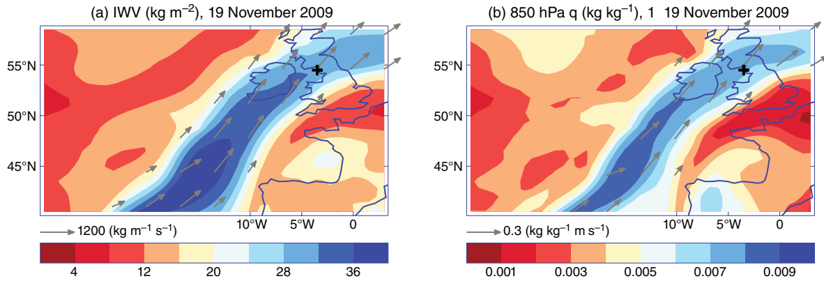
Figure 1. ERA Interim moisture and moisture transport fields associated with the heaviest daily rainfall event in the GPCP-1DD record (1996–2013) over the Cumbrian region (denoted by +): (a) column-integrated water vapour (IWV, \text{kg m}^{-2} , colours) and integrated water vapour transport (arrows show direction and length denotes magnitude, shown only for values greater than 400 \text{ kg m}^{-1} \text{ s}^{-1} ), (b) 850 hPa specific humidity ( q in \text{kg kg}^{-1} , colours) and vapour transport (arrows, plotted for V_T > 0.1 \text{ (kg kg}^{-1}) \text{ (m s}^{-1}) ).
