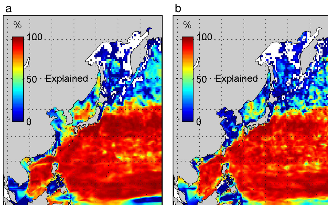
Figure 8. Percentage of the interannual variability of (a) A_a and (b) A_{sa} for \eta\text{-}\eta_{IB} explained by that of \eta_{ster} over 1900–2010, derived from SODA. Blank areas indicate the grids where the correlation of the interannual variability of A_a or A_{sa} between \eta\text{-}\eta_{IB} and \eta_{ster} are not significant at 95% confidence level.
