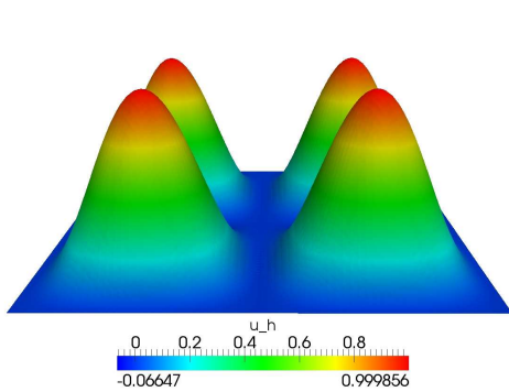
(a) Finite element approximation to (5.1).
