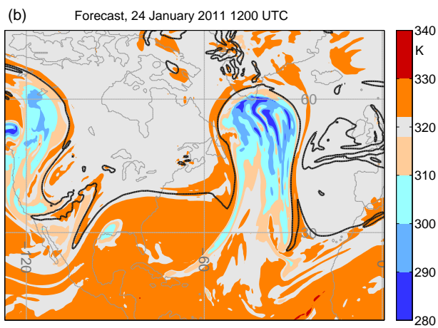
Figure 10: As in Fig. 6, but for the 320-K isentropic surface and for the period 12 UTC 22 January 2011 to 1200 UTC 24 January 2011.
