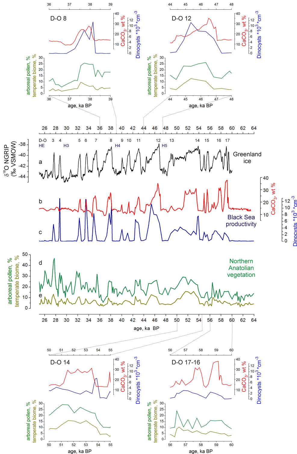
Fig. 6. Northern Anatolian vegetation and the Black Sea productivity in response to D–O and HE climatic variability: (a) \delta^{18}\text{O} record ( \text{‰ VSMOW} ) from NGRIP (GICC05) ice core (Svensson et al., 2008) with numbers of GI and HE marked above the curve; (b) calcium carbonate record from core 25-GC1 (wt %); (c) total dinocyst concentration from core 25-GC1 (specimens \times 10^3 \text{ cm}^{-3} ); (d) arboreal pollen (%) and (e) temperate biome (%) from core 25-GC1. The longest GI 17–16, 14, 12 and 8 are plotted in extra graphs, demonstrating a good correlation of northern Anatolian vegetation with the Black Sea productivity records.
