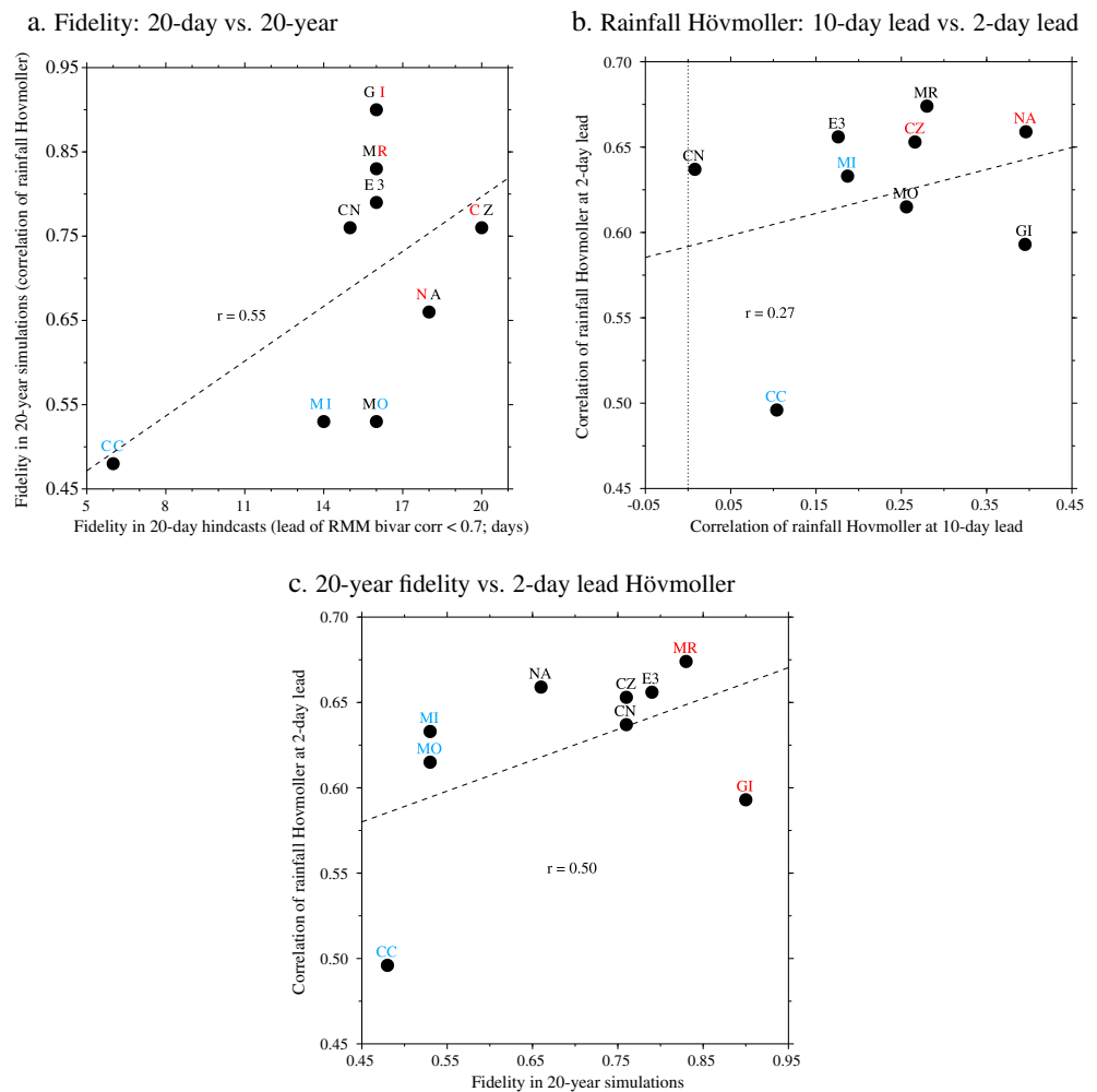
Figure 1. For each model, (a) MJO fidelity in 20 day hindcasts against fidelity in 20 year climate simulations; (b) pattern correlations of Hövmoller diagrams of daily mean rainfall (averaged 10°S–10°N and computed over 60°–160°E) between TRMM and the model, at 2 day and 10 day lead times; (c) fidelity in 20 year climate simulations against the 2 day pattern correlations from Figure 1b. In Figure 1a, the color of the first letter of each code gives relative fidelity among all thirteen 20 day hindcast models (blue: lower tercile; black: middle tercile; red: upper tercile); the color of the second letter gives relative fidelity among all twenty-seven 20-year climate simulation models (blue: lower 25%; black: middle 50%; red: upper 25%). In Figure 1b, the codes show 20 day hindcast fidelity; in Figure 1c, they show fidelity in 20 year climate simulations. The least-squares regression lines and correlation coefficients are also shown. Without CanCM4 (CC) the correlation in Figure 1a is 0.32.
