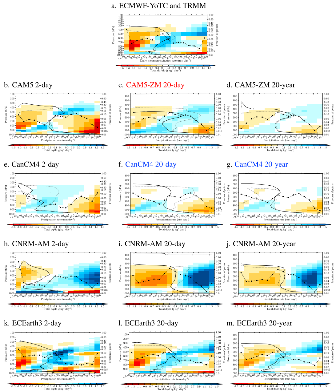
Figure 5. (a–ab) Models and experiments describing data as follows: Shading shows the mean vertical profiles of the rate of change of specific humidity ( dq/dt ; g\ kg^{-1}\ day^{-1} ) for each range of rain rates on the horizontal axis. Solid (dotted) lines are zero contours of the dq/dt from GCM dynamics (physics). Dynamics tendencies are positive (moistening) above and to the right of the solid line; physics tendencies are positive below and to the left of the dotted line. Dashed lines show probability distribution functions (PDFs) of rain rates, using the right-hand vertical axis. Composites are computed from time step data for 2 day hindcasts, 3 h data for 20 day hindcasts, and 6 h data for 20 year climate simulations. For 20 day hindcasts and 20 year climate simulations, colored panel labels indicate MJO fidelity. Note that Figure 5a is repeated for ease of comparison.
