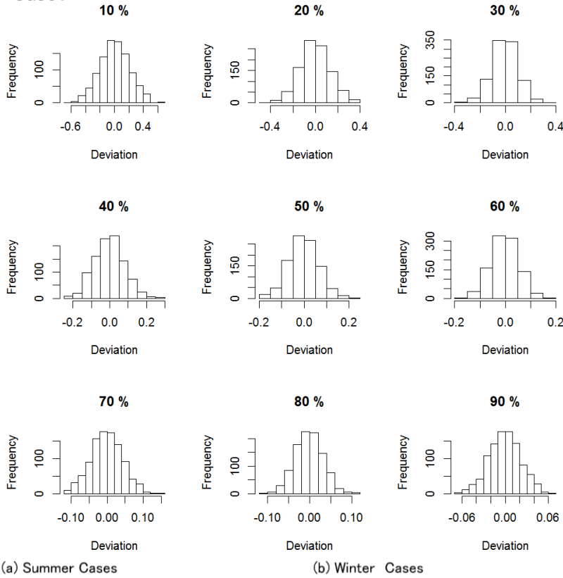
Fig. 4 Histograms of temperature deviation (sampled mean temperature - original mean temperature) (°C) in random sampling (Case 1, Table 1). Compare with Fig. 2a (case 1) when 100 % of the data are used to show the actual values. Frequency is the number of a particular temperature deviation with all subplots having 1000 samples. The number above each subplot indicates the percentage of sensors (from the original 183) randomly sampled to be analysed for statistics to be calculated.
