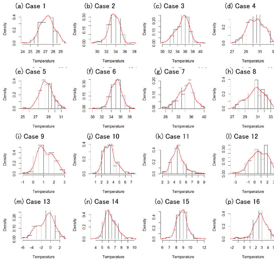
Fig. 2 Histograms of original temperature (°C) distribution when 183 (summer, cases 1-8) and 200 (winter, cases 9-16) sensors are used. See Table 1 for details of each case.
