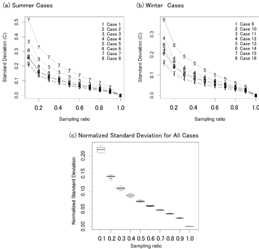
Fig. 5 Standard deviation (°C) of mean temperature (from the 1000 samples) and normalized standard deviation (the standard deviation of mean temperature divided by the original standard deviation) with changing proportion of sensors present. Numbers on lines refer to the case number. See Table 2 for more details.
