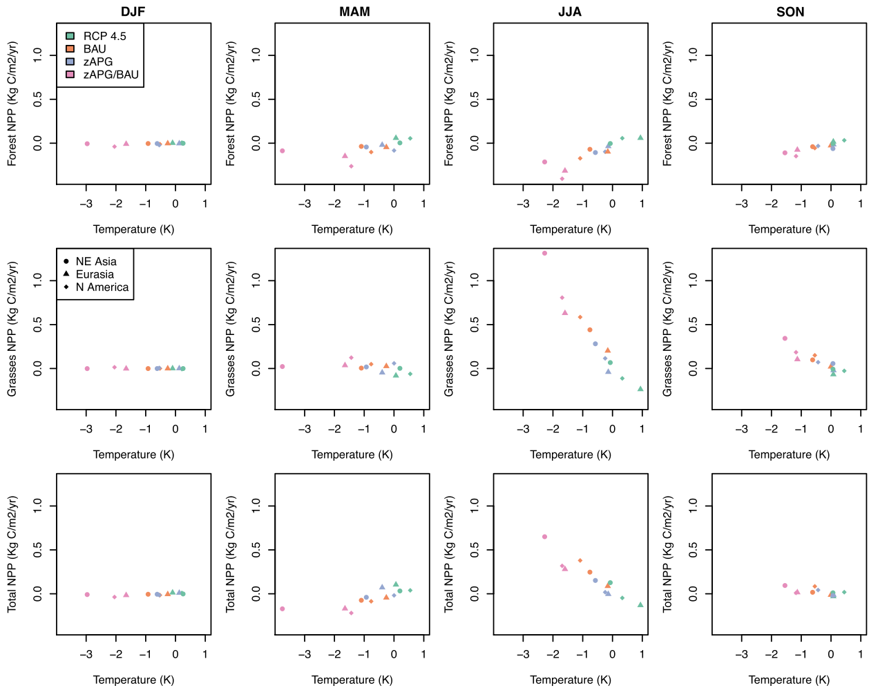
FIG. 4. The seasonal pattern in the relationship between changes in NPP and changes in temperature in the midlatitudes for (top) broadleaf and needleleaf trees, (middle) C_3 and C_4 grasses, and (bottom) all plant functional types. The anomaly is for the last 10 years of the simulations minus the same period for the No LUC control. Regions used here can be found in Fig. 1e. SON denotes the NH fall season (September–November).
