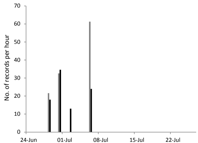
Figure 4. The frequency of territorial acquisition behaviours (grey bars) and courtship behaviours (black bars) during morning observations from 24 June to 26 July 2010.
