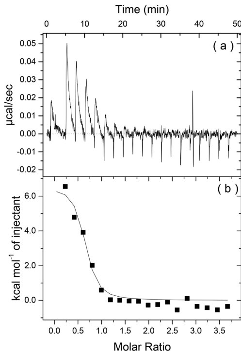
Fig. 2 (a) Heat release as a function of time and (b) energy released as a function of the molar ratio for Apo-I titrated with \text{C}_{16} -GGGRGDS.
