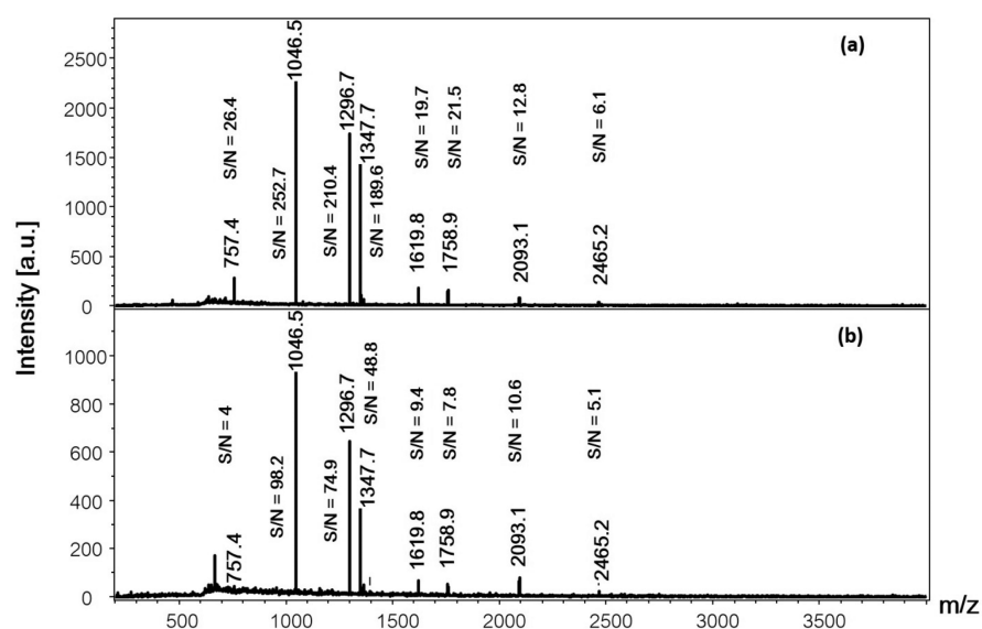
Figure 1. MALDI mass spectra of peptide standards mixture (1 fmol on an AnchorChip target) acquired on an Ultraflex TOF/TOF mass spectrometer using (a) CHCA and (b) CICCAs as matrix and the sample preparation protocol as recommended by the manufacturer. All observed peptide analyte [M + H]^+ ions are labeled with their recorded m/z and S/N values.
