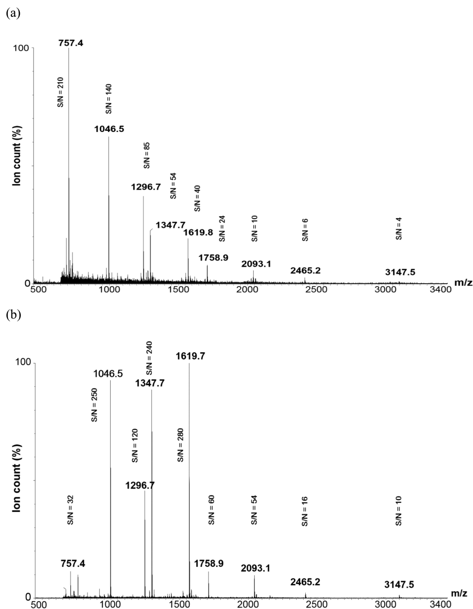
Figure 2. MALDI mass spectra of peptide standards mixture (20 fmol on a stainless steel target) acquired on a Q-TOF Premier mass spectrometer using (a) CHCA (100% intensity = 457 counts) and (b) CICCA (100% intensity = 1580 counts) as matrix and the sample preparation protocols for each matrix as reported by Leszyk. All observed peptide analyte [M + H]^+ ions are labeled with their recorded m/z and S/N values.
