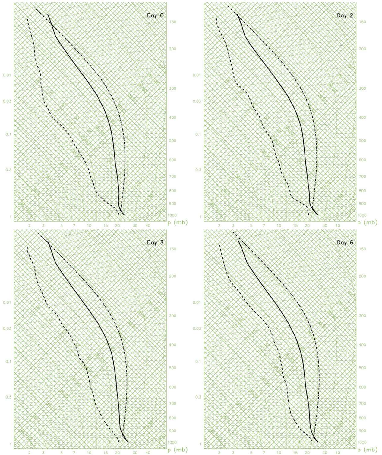
FIG. 8. Temperature and specific humidity profiles for column 1 of experiment 1. The profiles are plotted at (top left) day 0, (top right) day 2, (bottom left) day 3, and (bottom right) day 6.
