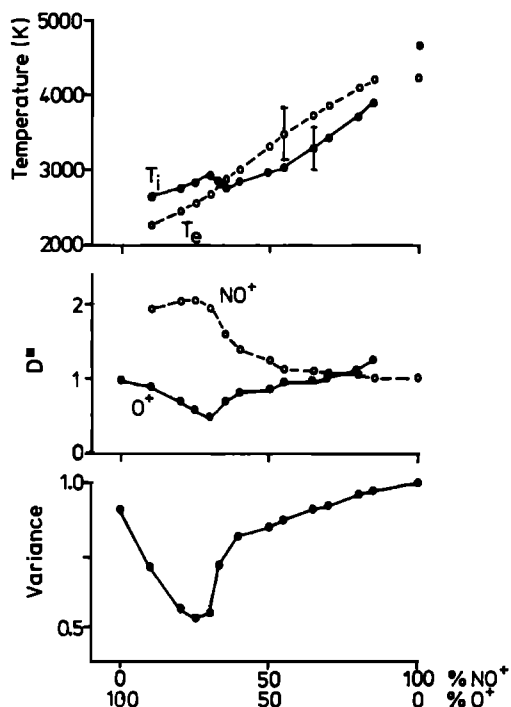
Fig. 5. Fitted values of (a) ion and electron temperature and (b) D^* for both atomic and molecular ions as a function of ion composition. These results were obtained from an analysis of the integrated spectrum obtained at 275 km in scan position 5 of the EISCAT CP-3-E experiment on August 27 (refer to Figure 1). The bottom panel shows the fit variance (arbitrarily normalized to unity at its maximum value) as a function of composition. The integration period was 110 s, and the aspect angle remained fixed at 62.7^\circ . The error bars represent the maximum uncertainty obtained in the derived parameters.
