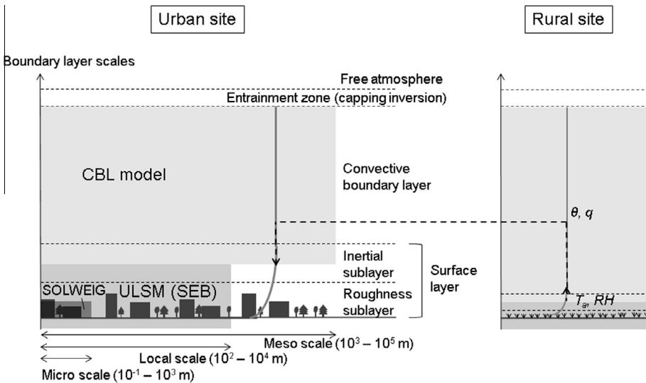
Fig. 1. Relation between boundary layer scales, the models and observations in this study: the convective boundary layer (CBL), surface energy balance (SEB) and micro-scale radiation environment (SOLWEIG), urban land surface model (ULSM).
