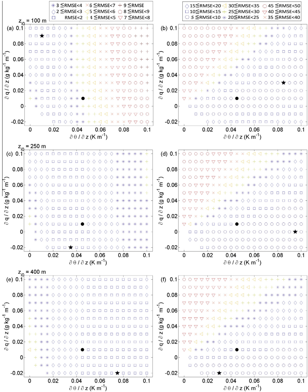
Fig. 11. Root Mean Square Error (RMSE) (left) air temperature ( T_a ), and (right) relative humidity (RH) for initial convective boundary layer ( z_{i0} ) (a, b) 100 m, (c, d) 250 m (e, f) 400 m for different combination of initial vertical gradients of potential temperature ( \partial \theta / \partial z on x-axis) and specific humidity ( \partial q / \partial z on y-axis): sensitivity test B4 (Table 3c) of BLUEWS. The closest point to average values of \partial \theta / \partial z (=0.043 \text{ K m}^{-1}) and \partial q / \partial z (=0.009 \text{ g kg}^{-1} \text{m}^{-1}) is indicated by a black dot ( \bullet ) and minimum RMSE by a star ( \star ).
