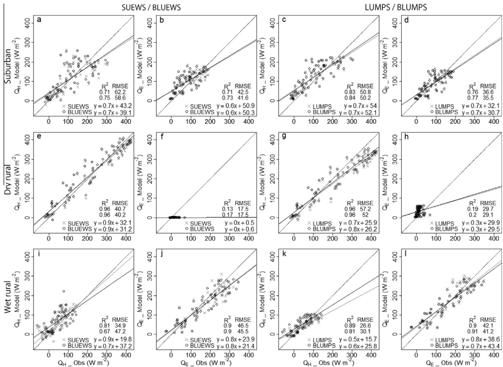
Fig. 4. Modelled sensible and latent fluxes ( Q_H, Q_E ) (1 h) versus the observations for uncoupled (LUMPS, SUEWS, grey) and coupled (BLUMPS, BLUEWS, black) runs for (a–d) suburban (e–h) dry rural and (i–l) wet rural. Model statistics ( R^2, RMSE , linear regression) are shown.
