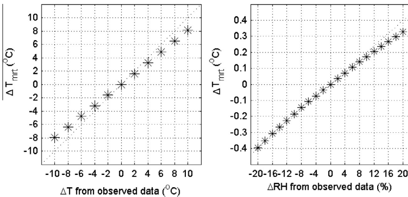
Fig. 7. Change in calculated mean radiant temperature ( T_{mrt} ) for the S0 run to changes in (left) air temperature ( T_a ) (S1) and (right) relative humidity (RH) (S2) (see Table 3a and Section 5.1).
