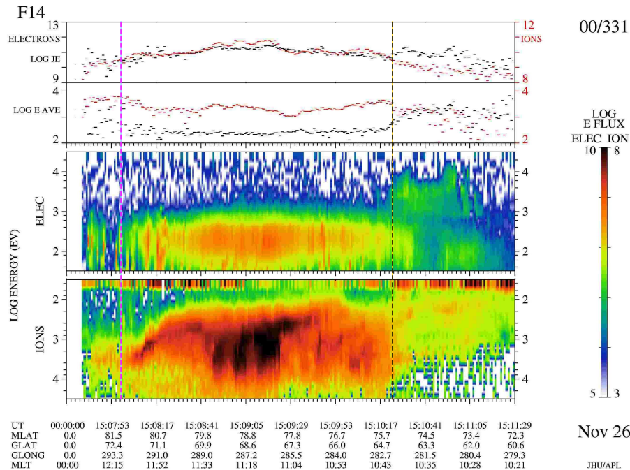
Fig. 6. DMSF F14 observations of the cusp pass around the 12 MLT meridian at 15:07:58–15:10:27 UT. The top panel shows the integrated energy flux of electrons (in black) and ions (in red). The second panel shows the corresponding average energies. The upper spectrogram shows the differential energy flux of electrons, contoured as a function of energy and observation time. The bottom panel shows the same for ions, with the ion energy scale inverted. The blue and mauve dashed line gives the poleward edge of the cusp precipitation and the orange and black dashed line gives the equatorward edge.
