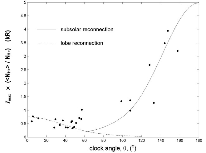
Fig. 10. Scatter plot of the normalised peak Lyman- \alpha emission intensity, I_{\max}\{\langle N_{\text{H}^+} \rangle / N_{\text{H}^+}\} , where N_{\text{H}^+} is the proton data seen by ACE and \langle N_{\text{H}^+} \rangle is its average value over the interval 15:00–16:00. The normalised intensities are averaged over 12:00–12:30 MLT and are plotted against the IMF clock angle in GSM observed by ACE, \theta (points). The ACE data have been lagged by the derived ACE-to-Earth propagation delay \delta t_E . The solid line shows the variation predicted by the cusp model for a subsolar reconnection site, the dashed line is the variation predicted for the same model inputs and a lobe reconnection site.
