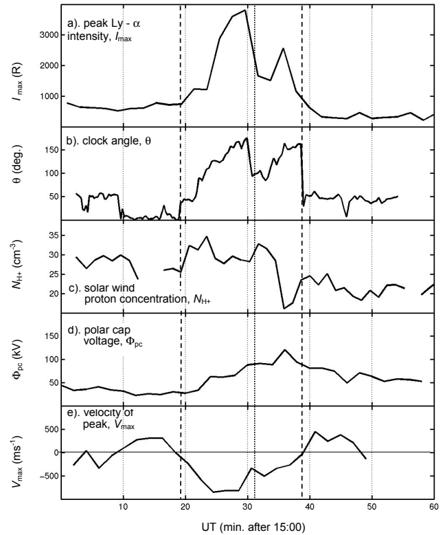
Fig. 7. Variations of parameters observed during the brief intensification of the cusp aurora: (a) I_{\max} , the peak Doppler-shifted Lyman- \alpha emission intensity seen along the meridian keogram from SI-12/FUV data integrated over 12:00–12:30 MLT (Fig. 5); (b) \theta , the IMF clock angle in GSM coordinates, as observed by ACE; (c) N_{\text{H}^+} , the proton concentration in the solar wind seen by ACE; (d) \Phi_{\text{pc}} , the transpolar voltage from the model fit to the SuperDARN radar data; and (e) V_{\max} , the meridional phase velocity of motion of the peak Lyman- \alpha emission. All ACE data have been lagged by the derived ACE-to-Earth propagation delay \delta t_E .
