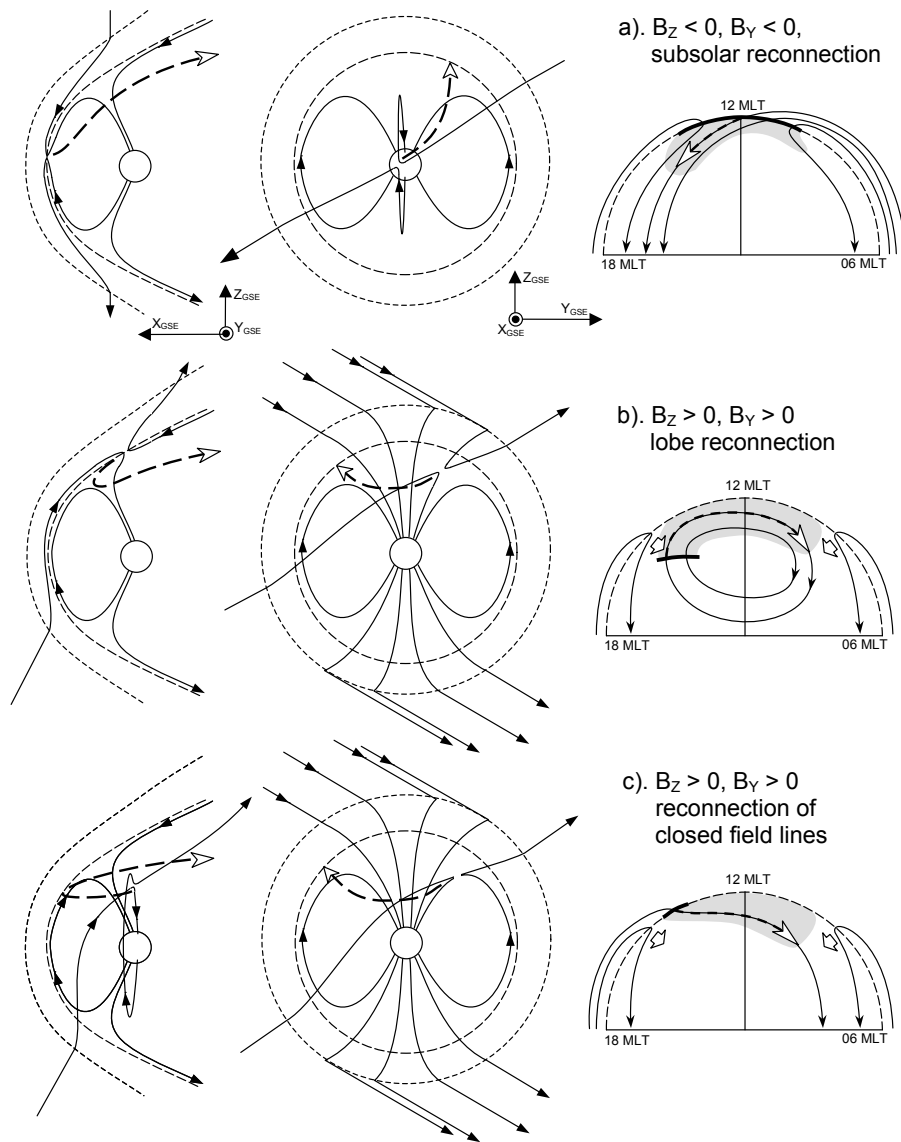
Fig. 11. Schematic illustrations of the reconnection geometry for (a) a subsolar reconnection site with IMF B_z < 0 , B_y < 0 , (b) a lobe reconnection site with IMF B_z > 0 , B_y > 0 and (c) a dusk-flank reconnection site on closed field lines with IMF B_z > 0 , B_y > 0 . The left-hand figures are views of the noon-midnight meridian from the dusk flank, the centre figures are views of the dayside from the Sun; in these columns, thin lines with arrows are magnetic fields and the dashed arrow gives the evolution of newly-reconnected flux. The right-hand figures are views looking down on the northern polar cap with 12 MLT at the top of each, the grey area is newly-reconnected flux where cusp precipitation is seen. In this right-hand column, thin lines with arrows are flow streamlines, the dashed lines are non-reconnecting segments of the open-closed field line boundary (OCB), thick lines are the ionospheric projections of active reconnection sites, and open arrows show the OCB motion.
