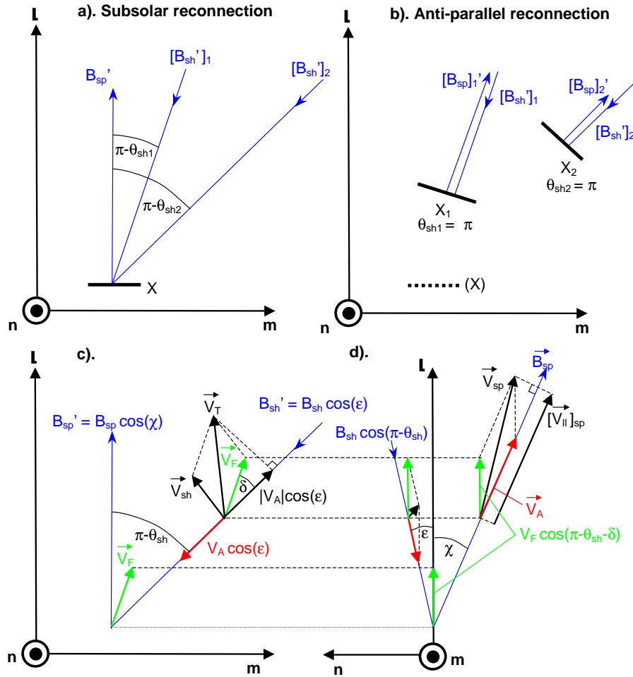
Fig. 13. Geometry of newly-opened field lines at the dayside magnetopause. (a), (b), and (c) show the l - m plane of the magnetopause, whereas (d) shows a cross section of the magnetopause in the l - n plane, where n is the outward normal to the boundary. (a) shows two orientations of the sheath field (projections onto the l - m plane are [B_{sh}']_1 and [B_{sh}']_2 ) for component reconnection at a reconnection site X . (b) shows schematically reconnection sites X_1 and X_2 needed to give anti-parallel reconnection for the same sheath field orientations. (c) and (d) give the geometrical construction (projected onto the l - m and n - l planes, respectively) needed to compute field line motion and the proton acceleration on crossing the magnetopause RD.
