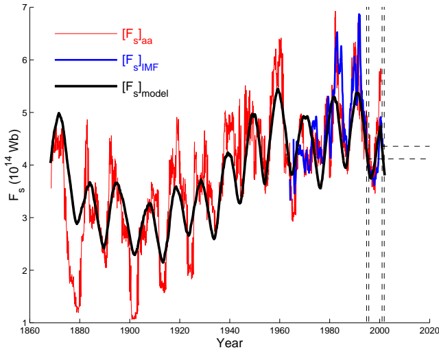
Fig. 3. The variation of open solar flux F_s since 1868. The blue line shows monthly means deduced from IMF observations [F_s]_{\text{IMF}} = 2\pi r_1^2 |B_{r1}| , whereas the red curve shows 1-year values [F_s]_{\text{aa}} deduced from the aa geomagnetic index using the method of Lockwood et al. (1999) (see Fig. 2 for a more detailed view of the last 3 cycles). The black curve shows the best fit [F_s]_{\text{SM}} using the open flux continuity model of Solanki et al. (2000). The vertical dashed lines mark the times of the two perihelion passes by Ulysses and the horizontal dashed lines the mean open flux deduced during those passes. Note that the model parameters were obtained from a best fit to data for up to 1986 and thus the values for the two perihelion passes are predictions that match the Ulysses observations very well in both cases.
