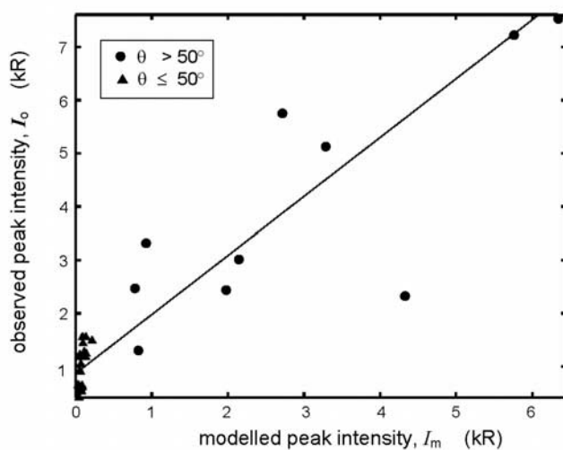
Figure 8. Scatter plot of I_o against I_m for the lag giving peak correlation shown in Figure 7 and the best-fit linear regression fit. Symbols differentiate between data taken when the IMF clock angle is smaller than or exceeds 50^\circ .
