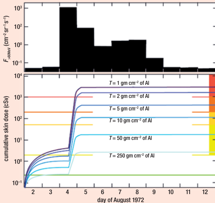
9 (a): The variation of daily mean values of the flux of protons with energies exceeding 60 MeV during the August 1972 SEP event (the largest event in figure 3). (b): The growth on the cumulative skin dose behind aluminium shields of thickness (from dark to light blue) 1, 5, 10, 50 and 250 gm cm -2 . The thresholds used in figure 3 are also given, using the same colour scheme.
