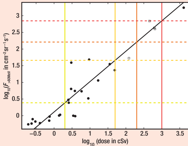
4: Scatter plot of modelled cumulative-event skin dose behind a shield of 1 gm cm -2 of aluminium as a function of the peak value of the daily means of proton flux (E > 60 MeV) during the event. The solid points are the events during the era of the Apollo missions, the open squares are values derived during some of the larger events seen in recent years. The thresholds used in figure 3 are also given, using the same colour scheme.
