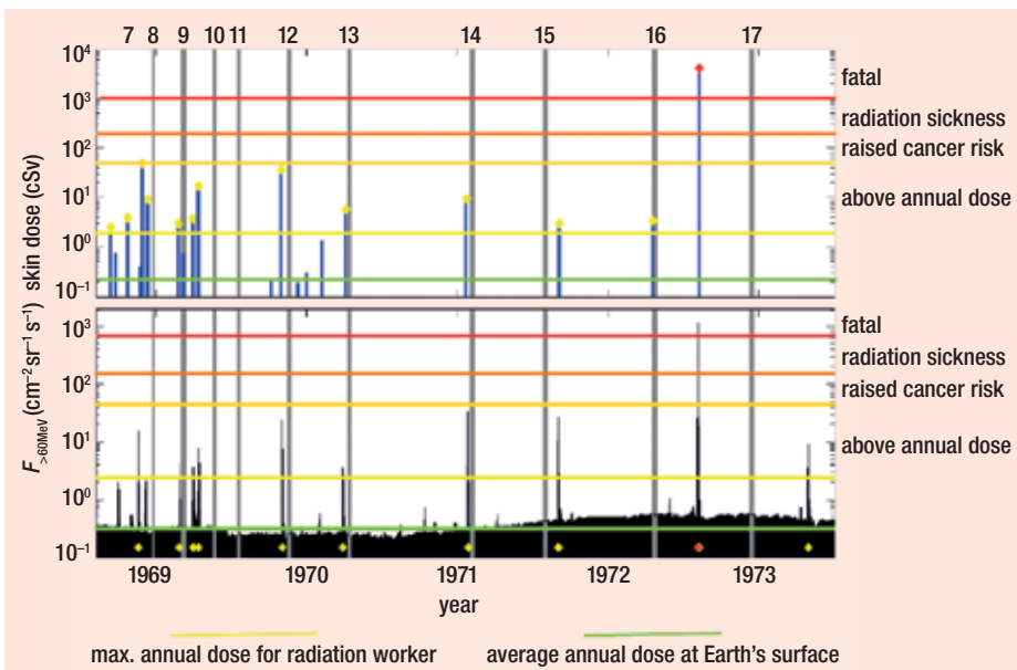
3: The variation of (top) cumulative-event skin dose behind a shield of 1 gm cm -2 of aluminium and (bottom) the flux of >60 MeV protons, both in interplanetary space. In both cases, the scale is logarithmic. The vertical grey bars give the times when the Apollo astronauts were outside Earth's magnetosphere in interplanetary space (the missions are numbered along the top). The horizontal lines show: in green, the average annual dose at the Earth's surface; in yellow, the maximum annual dose allowed for an employee working with radiation; a threshold for seriously enhanced long-term risk of cancers; in brown, a threshold above which most individuals will suffer severe radiation sickness and in red, a threshold above which doses are potentially fatal. These thresholds have been mapped onto the lower panel using the scatter plot presented in figure 5.
