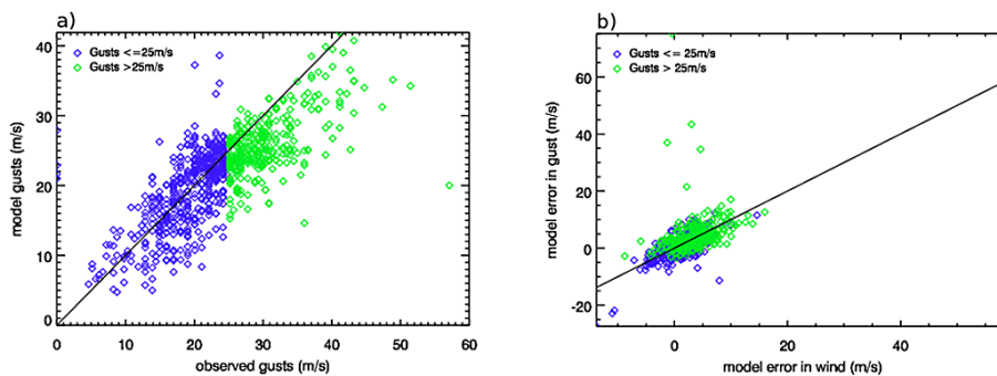
Figure 9. (a) Scatter plot of model gust against observed gust for the storm Anatol, for stations with altitudes \leq 500 m only. (b) Plot of error in model gust (model gust – station gust) vs. error in model wind at each of the stations that recorded both gusts and winds also for Anatol. In both plots points representing stations which recorded gusts greater than 25 \text{ m s}^{-1} are plotted in green, and the solid line represents y = x .
