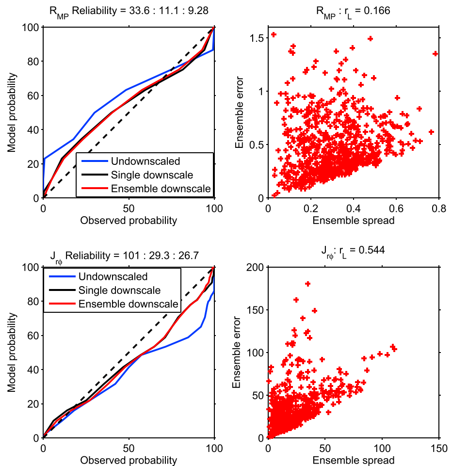
Figure 7. (left) Reliability diagrams for (top) R_{MP} and (bottom) J_{r0} resulting from undownscaled, single downscale, and ensemble downscale model-like time series. (right) Ensemble spread error diagrams. See text for discussion.
