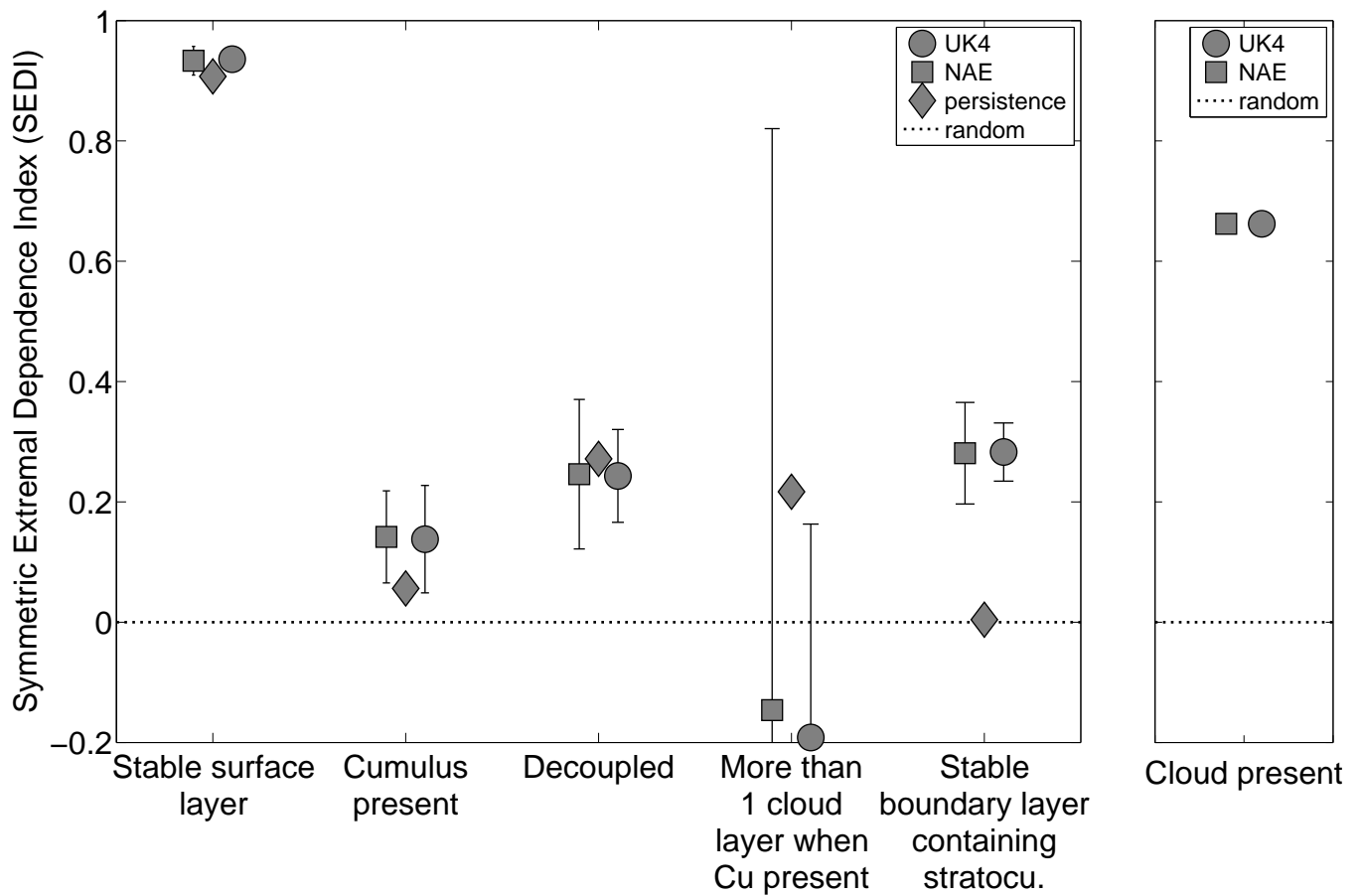
Figure 8. Summary of the SEDI score for each decision for the modal UK4 boundary-layer type and NAE boundary-layer type closest to the CFARR with 95% confidence intervals calculated using the forecast lead time data for the period 01/09/2009 - 31/05/2010. The right panel shows the SEDI score for the presence of cloud (>10%) below 3 km for the same period for the UK for the closest grid point to CFARR.
