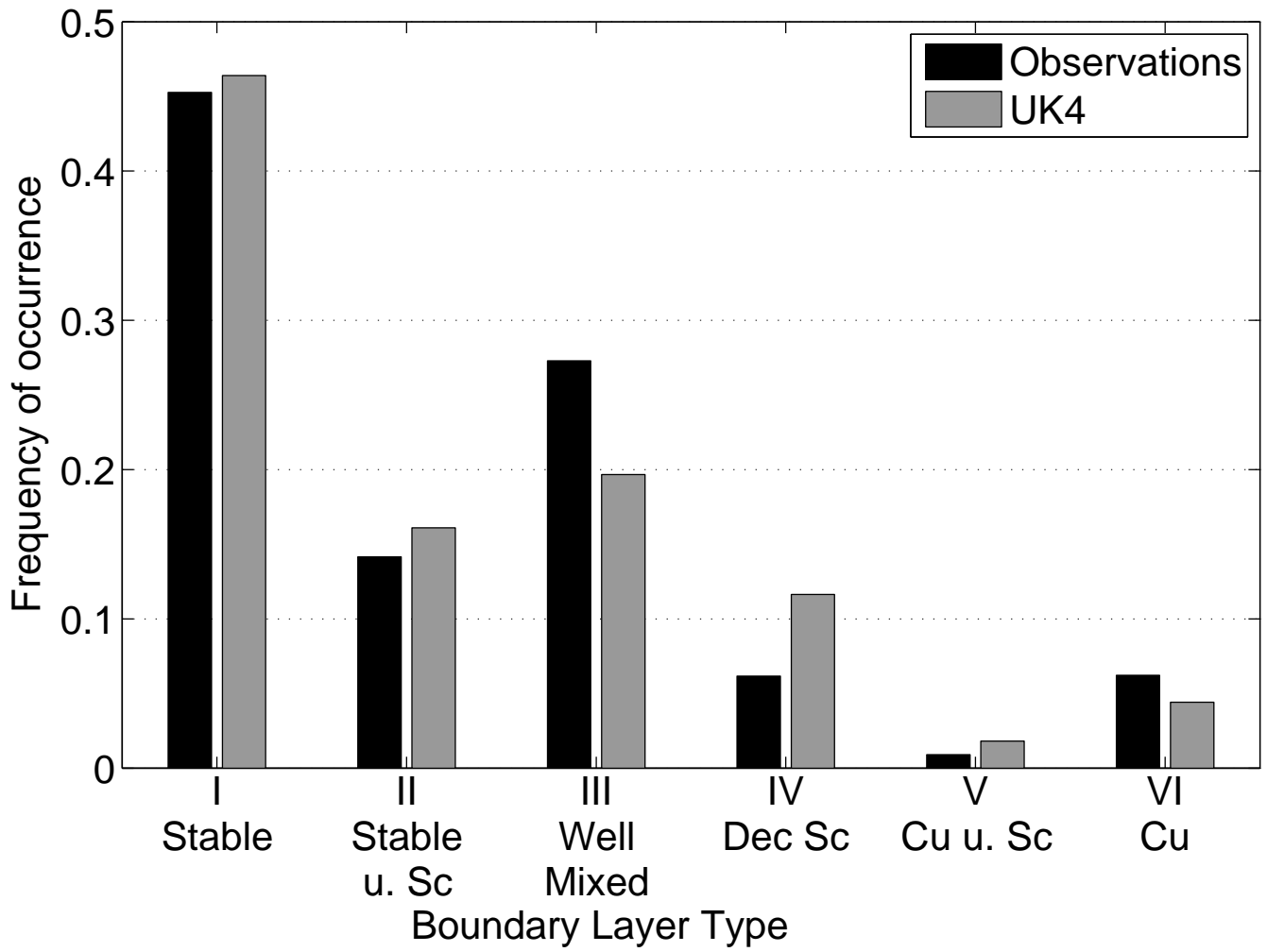
Figure 1. The frequency of occurrence of hourly boundary-layer types for the UK4 and the observations during the period 01/09/2009–31/08/2011.
