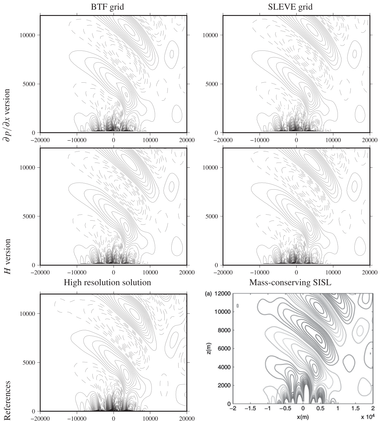
FIG. 6. Vertical velocity after 5h for the flow over a Schär et al. (2002) mountain on (left) the BTF and (right) SLEVE grids using both model versions with implicit gravity waves: (top) \partial p/\partial x and (middle) H versions, and (bottom) reference. Contours are 5 \times 10^{-2} \text{ m s}^{-1} , negative contours are dashed, and there is no zero contour. Here, \Delta t = 8 \text{ s} , N\Delta t = 0.08 . Comparison with a high-resolution solution ( \Delta x = 125 \text{ m} , \Delta z = 75 \text{ m} , \Delta t = 2 \text{ s} ) and with the semi-implicit, semi-Lagrangian solution presented by Melvin et al. (2010).
