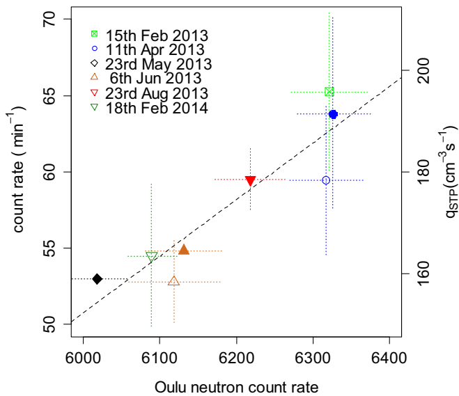
Fig. 7. Comparison between count rates obtained at the Regener–Pfotzer maximum (as identified using the spline method), and surface neutron monitor data from Oulu. Error bars in the geigeronde data represent the spread of the two tubes, and the error bars in the neutron monitor two standard errors during the 30 min period centred on the time when the Regener–Pfotzer maximum was reached. (Solid points represent ascent data, hollow points represent descent data.)
