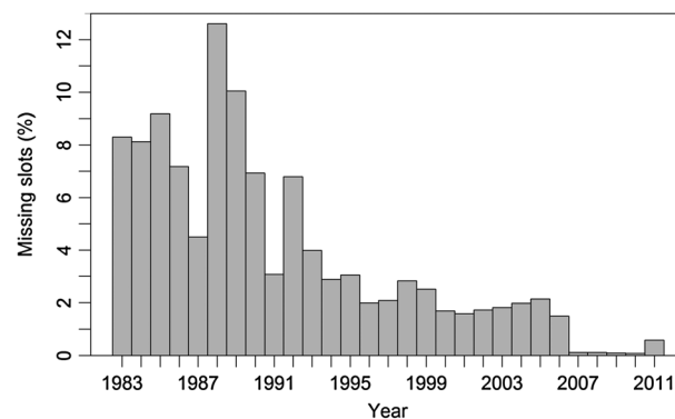
Figure 2. The annual percentage of missing TIR time slots calculated as the percentage difference between existing slots (i.e., images obtained from the Meteosat archive) and all possible slots.
