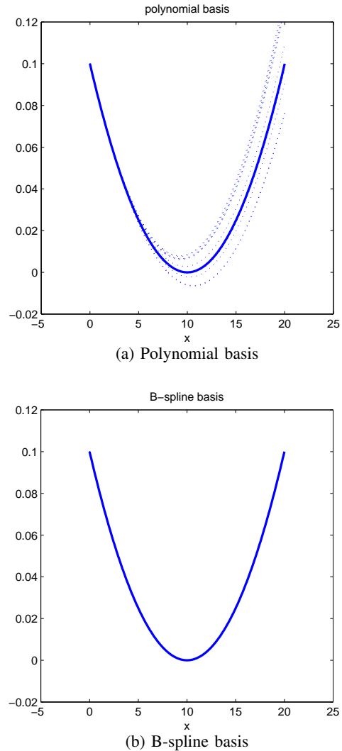
Fig. 2. Illustration of the superior numerical stability of the B-spline model over the polynomial model.
