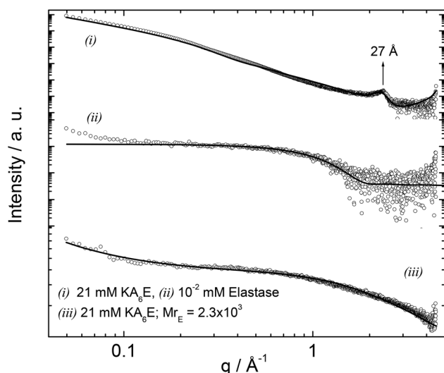
Fig. 8 SAXS curves measured for 21 mM \text{KA}_6\text{E} , M_{rE} = 2.3 \times 10^3 , in Trizma pH 8 and the corresponding controls. The full lines represent the fitting to the data as described in the text.
