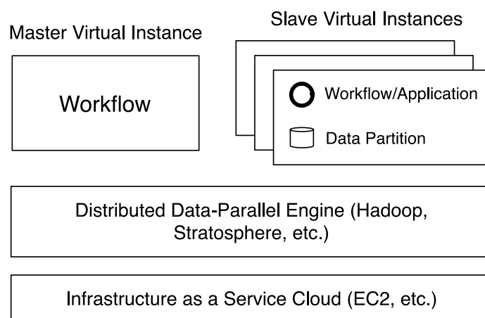
Figure 5: A framework for data intensive workflow applications in the Cloud.
