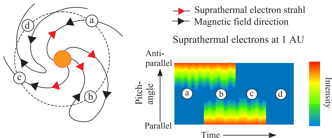
Figure 10: A sketch of heliospheric magnetic topology inferred from suprathermal electron observations. Left panel: A view of the ecliptic plane, with magnetic field lines shown as black arrows and the anti-sunward suprathermal electron flux shown as red arrows. Right panel: The STE pitch-angle distribution seen by a spacecraft in near-Earth orbit. At (a), the field is part of an inward-polarity sector, so the STE strahl is anti-parallel to the field. Similarly, at (c), the outward sector results in a parallel strahl. At (b), the magnetic field is connected to the Sun at both ends, resulting in both parallel and anti-parallel strahls, or counterstreaming. At (d), there is no solar connection, so no strahl is seen.
