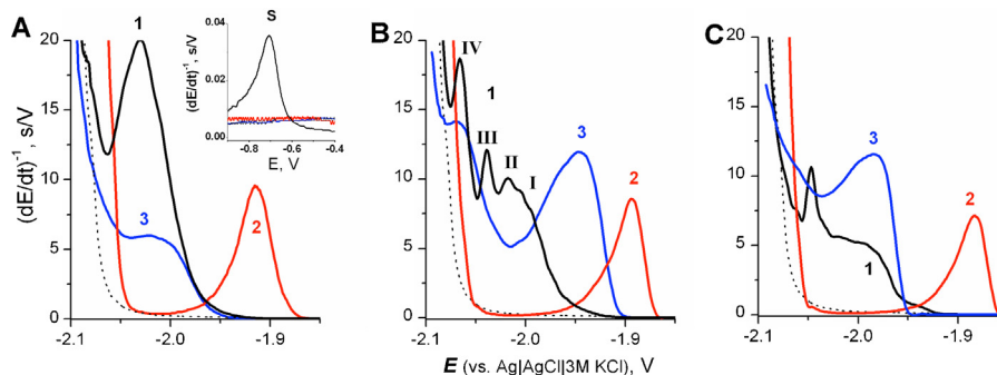
Fig. 1. CPS peaks H and S (inset) of YYKLVFFC (peptide 1 , black) YEVHHQKLVFF (peptide 2 , red) and KKLVFFA (peptide 3 , blue) at accumulation potential, E_A . (A) E_A = -0.1 V, (B) E_A = -0.9 V, (C) E_A = -1.3 V. Peaks were obtained in the presence of 2 \mu\text{M} peptides 1–3 in 35 mM phosphate buffer, pH 7.0 using HMDE at 25^\circ\text{C} ; t_A = 180 s; I_{\text{str}} = -11 \mu\text{A} ; background electrolyte (.....). (For interpretation of the references to color in the text, the reader is referred to the web version of the article.)
