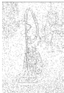
(f) Sobel
