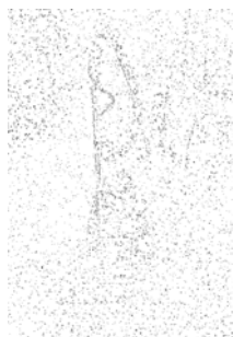
(p) Sobel
