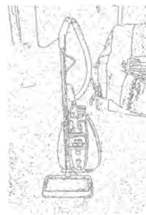
(i) SUSAN
