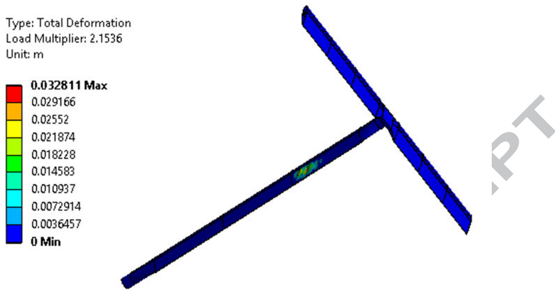
Figure 25. Buckling load multiplier and buckling mode shape of the blade
