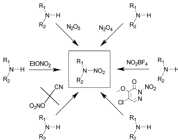
Figure 6: Nitrating agents
