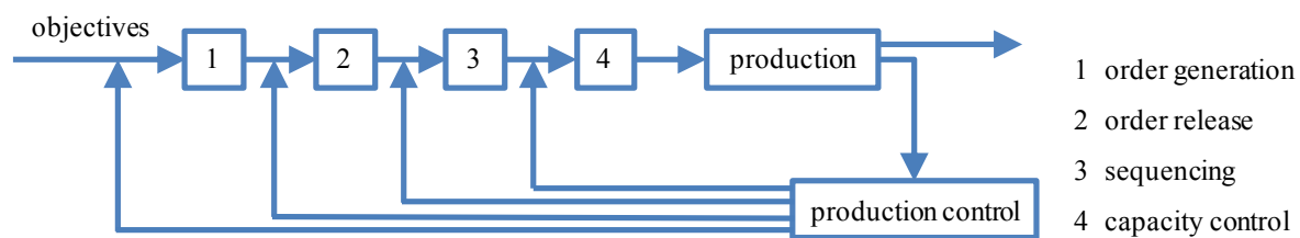
Figure 1: Cascaded closed-loop production control.
