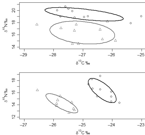
Figure 5. Stable isotope bi-plots for the River Lea where (○) Barbus barbus individuals, (Δ) Squalius cephalus individuals. Solid lines enclose the standard ellipse areas for each species, where black: B. barbus , dark grey: S. cephalus . Note differences in scales on all axes. Top all fish between 186 and 237 mm; Bottom: all fish between 400 and 435 mm.
