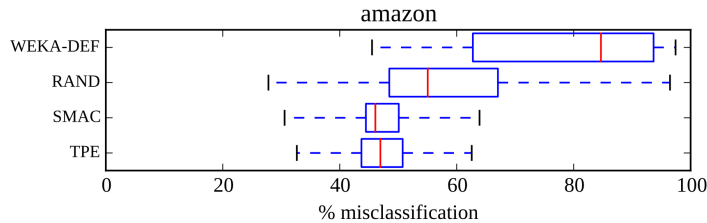
Fig. 3. Range of CV errors for ‘amazon’
