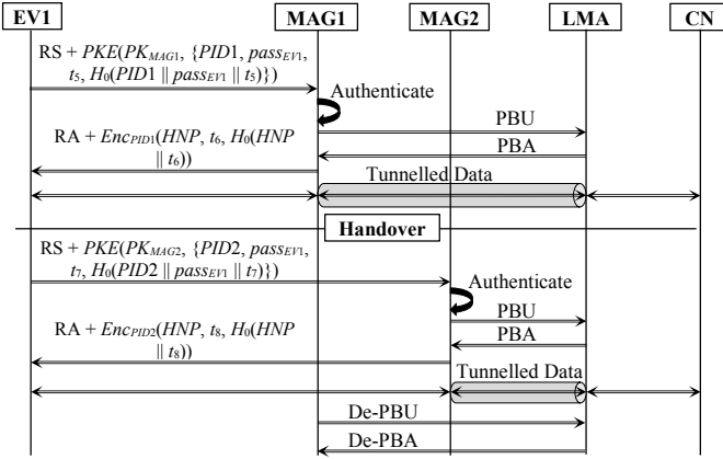
Fig. 3. SP-PMIPv6 Signalling Flow
